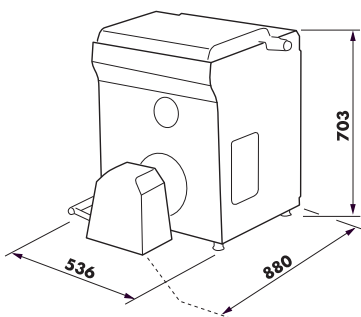
Dimensions TX98 Minimix
