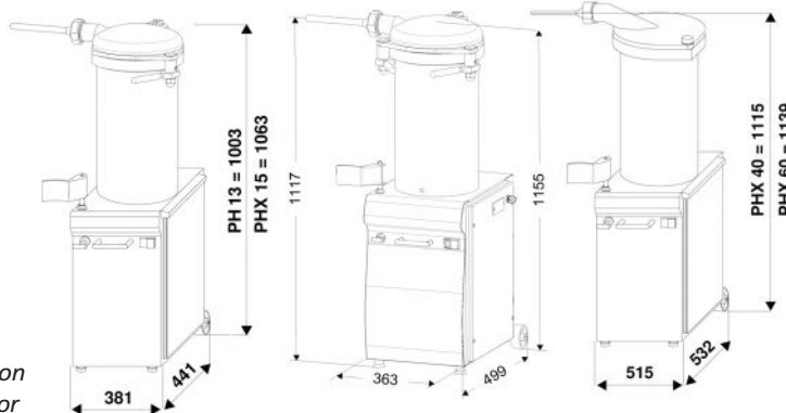
Dimensions PH13 - PHX15
