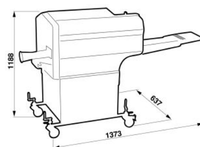
Dimensions PORTIO 140
